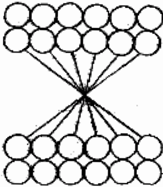
NEUTRON
